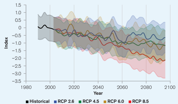
FIGURE 14. Projected Annual SPEI Drought Index, Namibia (Reference Period, 1986–2005) 89
