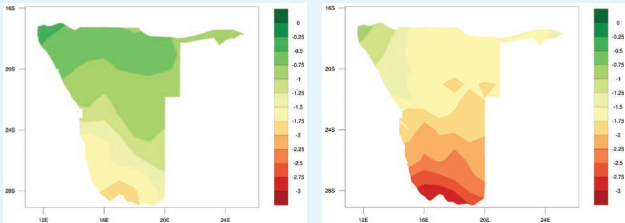
FIGURE 15. Projected SPEI in Namibia for the Periods 2040–2059 (left) and 2080–2099 (right) (RCP8.5, Reference Period, 1986–2005) 90
