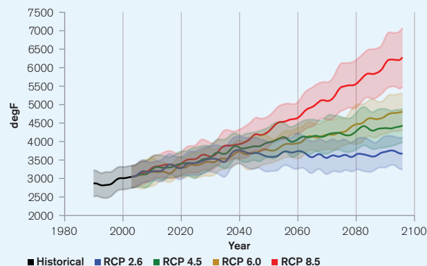
FIGURE 13. Change in cooling degree days (65°F) in Botswana for the period 2080–2099 89
