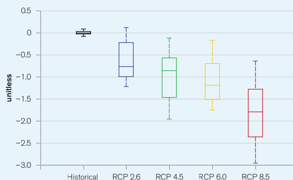
FIGURE 12. Annual SPEI Drought Index in Botswana for the period, 1986 to 2099 79
