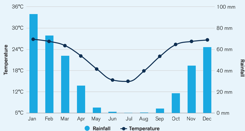
FIGURE 3. Average monthly temperature and rainfall for Botswana, 1991–2020 20
